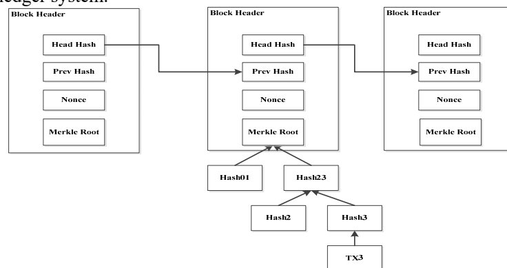
Fig.1 Blockchain Structure
